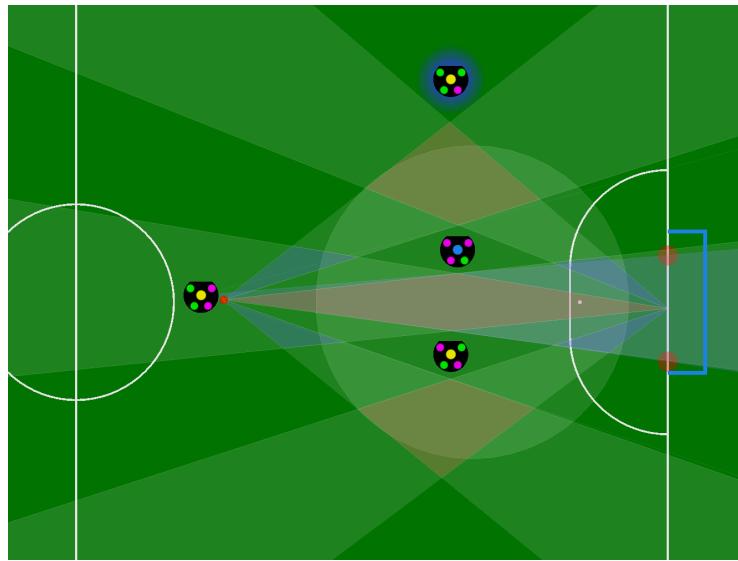
Fig. 7. Visualization of the assistant searching for a free spot for a pass. The red and blue areas show positions from where the robot can receive both the ball and shot at the goal.
